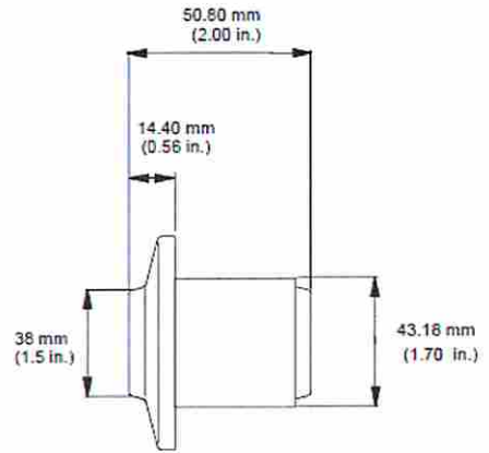
SHOCK MOUNT ASSEMBLY
